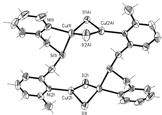
Fig. 3 Perspective view (crystallographic numbering) of 2 . Thermal ellipsoids are drawn at the 50% probability level. Selected bond lengths (Å) and angles ( ^\circ ): Cu(1)–N(1) 2.050(5), Cu(1)–S(1) 2.418(2), Cu(1)–I(1A) 2.649(1), Cu(1)–I(2A) 2.589(1), Cu(2)–N(2) 1.995(5), Cu(2)–I(1) 2.594(1), Cu(2)–I(2) 2.569(1), Cu(1) \cdots Cu(2A) 2.528(1); N(1)–Cu(1)–S(1) 85.6(2), N(1)–Cu(1)–I(2A) 111.6(1), S(1)–Cu(1)–I(2A) 124.61(6), N(1)–Cu(1)–I(1A) 116.0(1), S(1)–Cu(1)–I(1A) 98.40(5), I(1A)–Cu(1)–I(2A) 116.87(3), N(2)–Cu(2)–I(2) 122.5(1), N(2)–Cu(2)–I(1) 117.4(1), I(1)–Cu(2)–I(2) 119.63(3). (Symmetry code: A -x, -y, -z + 1 .)
