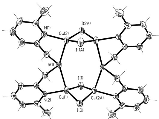
Fig. 1 Perspective view (crystallographic numbering) of 1 . Thermal ellipsoids are drawn at the 50% probability level. Selected bond lengths (Å) and angles ( ^\circ ): Cu(1)–N(2) 2.031(3), Cu(1)–S(1) 2.570(1), Cu(1)–I(1) 2.582(1), Cu(1)–I(2) 2.652(1), Cu(2)–N(1) 2.046(3), Cu(2)–S(1) 2.464(1), Cu(2)–I(1A) 2.586(1), Cu(2)–I(2A) 2.640(1), Cu(1) \cdots Cu(2A) 2.551(1); N(2)–Cu(1)–S(1) 82.47(9), N(2)–Cu(1)–I(1) 129.45(9), S(1)–Cu(1)–I(1) 108.14(5), N(2)–Cu(1)–I(2) 106.26(9), S(1)–Cu(1)–I(2) 100.88(4), I(1)–Cu(1)–I(2) 119.03(2), N(1)–Cu(2)–S(1) 84.79(9), N(1)–Cu(2)–I(1A) 125.11(9), S(1)–Cu(2)–I(1A) 111.83(4), N(1)–Cu(2)–I(2A) 107.85(9), S(1)–Cu(2)–I(2A) 99.29(4), I(1A)–Cu(2)–I(2A) 119.32(3). (Symmetry code: A -x + 1, -y + 1, -z + 2 .)
